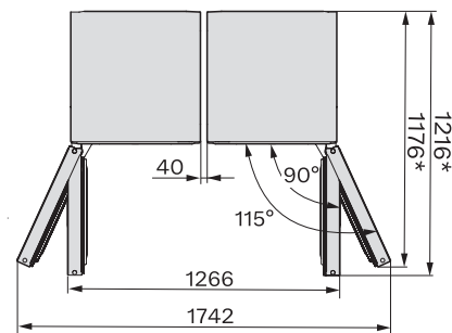
KS4383ED N, KS4383DD N, FNS4382E N, FNS4382D N, Nordic, installation sketch, Side-by-Side (*footnote) (drawings)
